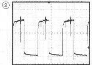
5.6 Vp-p 31.25kHz
