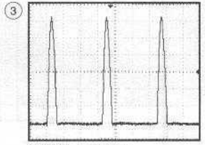
1.29 kV 31.25kHz
